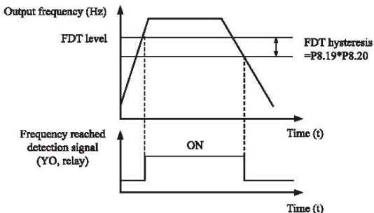
Figure 4-14 FDT level
